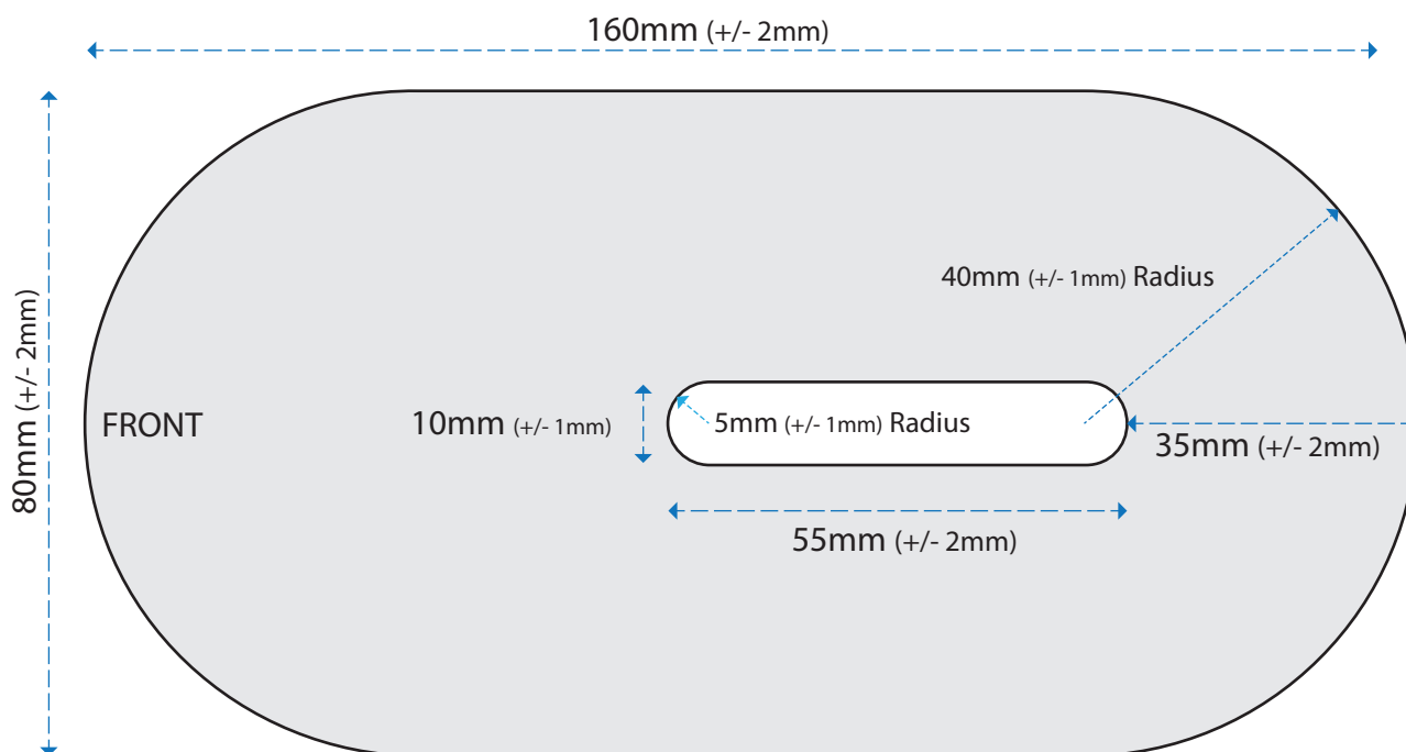
Diagram 1 Keelbox Sticker. (Note: This diagram is full size and can be used as a template if printed at 100%)
